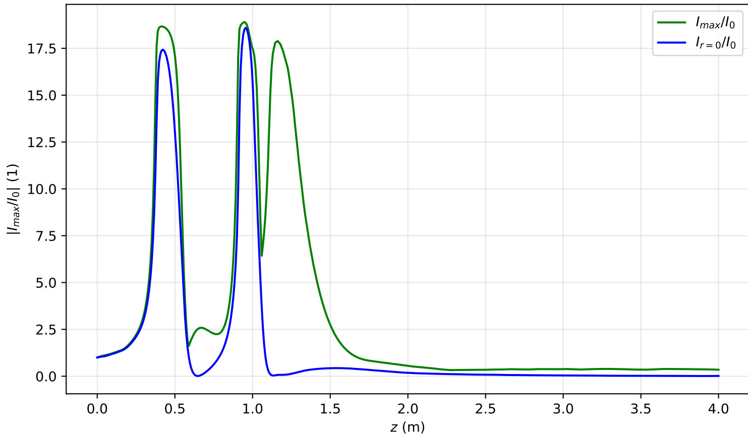
I_{max}(x = 0, y = 0, z)/I_0 , P_{in}=5.9P_{cr} , noisy input, artificial time
